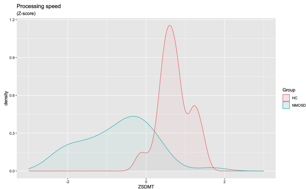
Figure 1. Processing speed.
